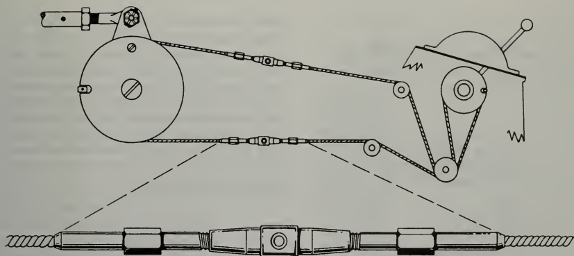
FIGURE 8-7. Engine control cable and turnbuckle assembly.
